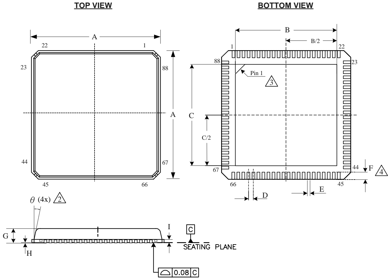
88 Pin QFN Package (10 x 10 mm)
