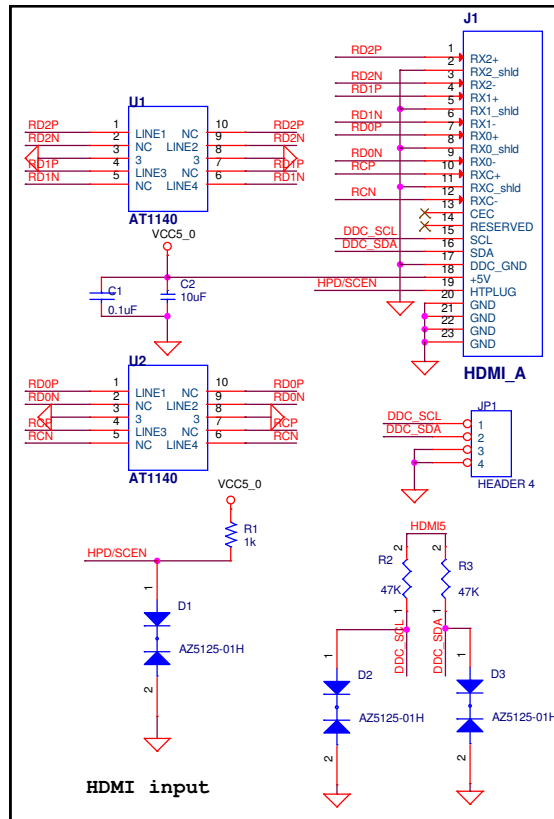
Figure 5(B): The connection of the HDMI inputs—CH7109A HDMI connectors
