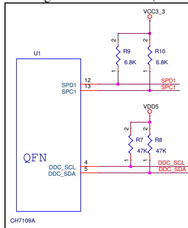
Figure 4: Serial Port Control
