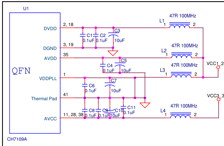
Figure 1: Power Supply Decoupling and Distribution
