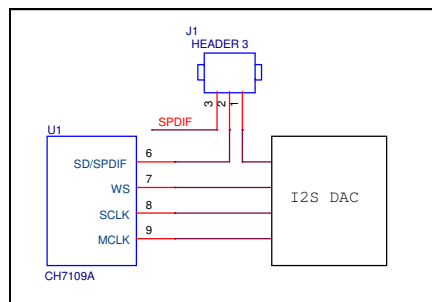
Figure 7: CH7109A IIS or SPDIF Output Pins
