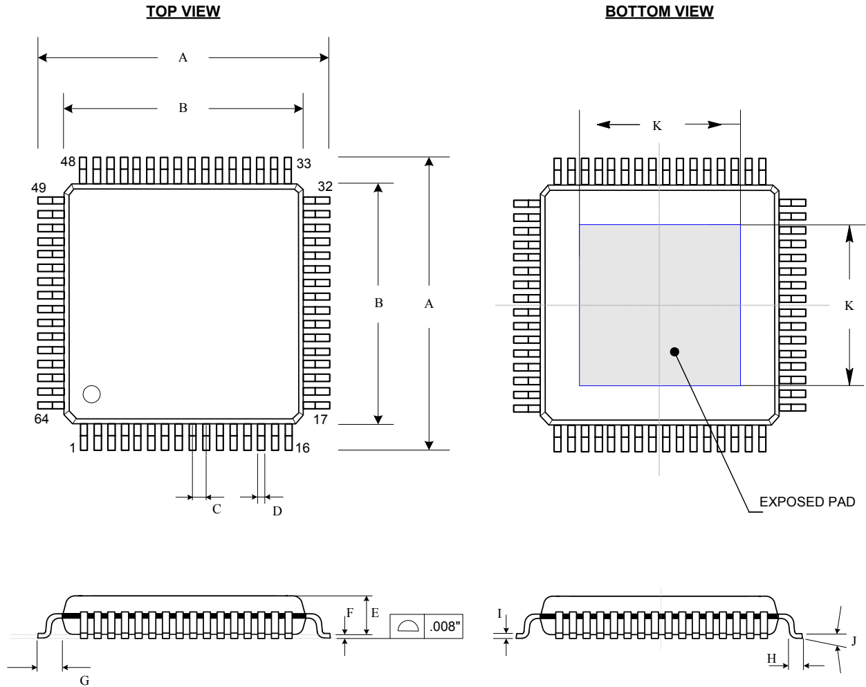
64 Pin LQFP (Exposed Pad) Package
