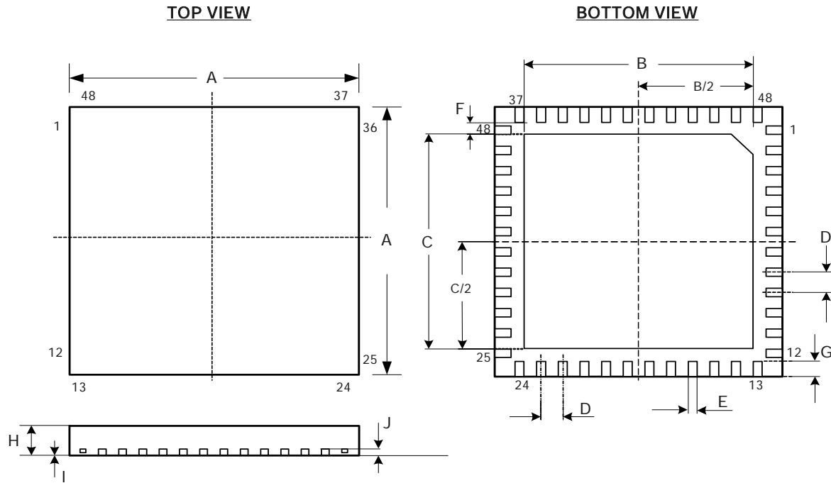
48 Pin QFN Package
