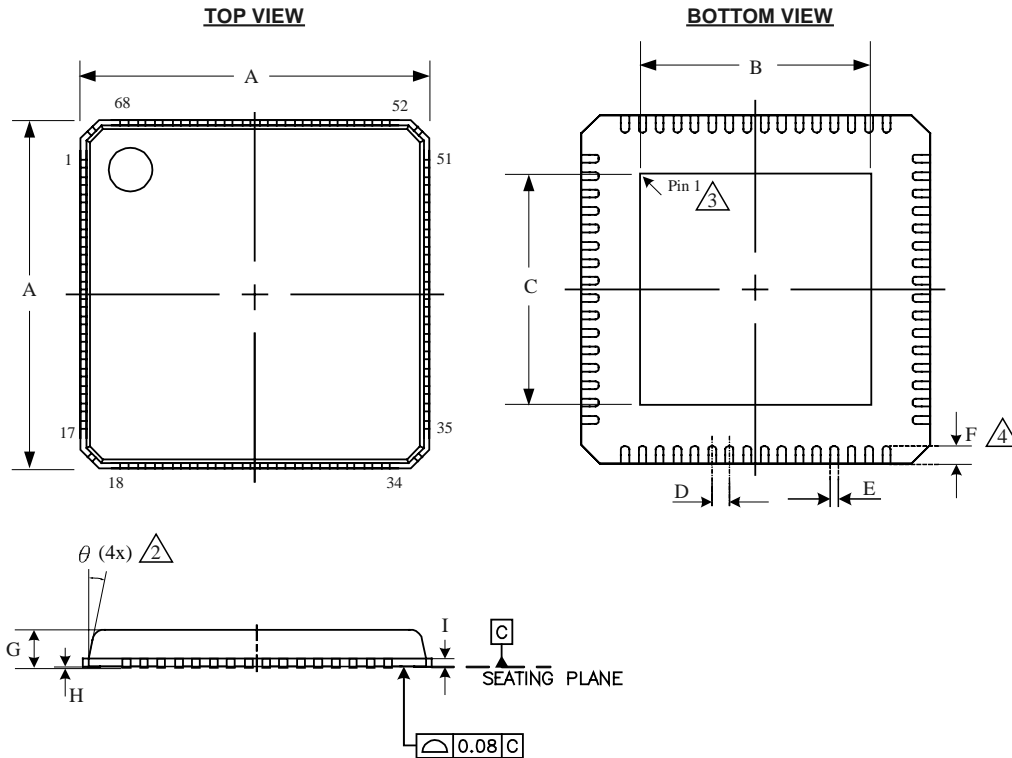
68 Pin QFN Package (8 X 8 mm)
