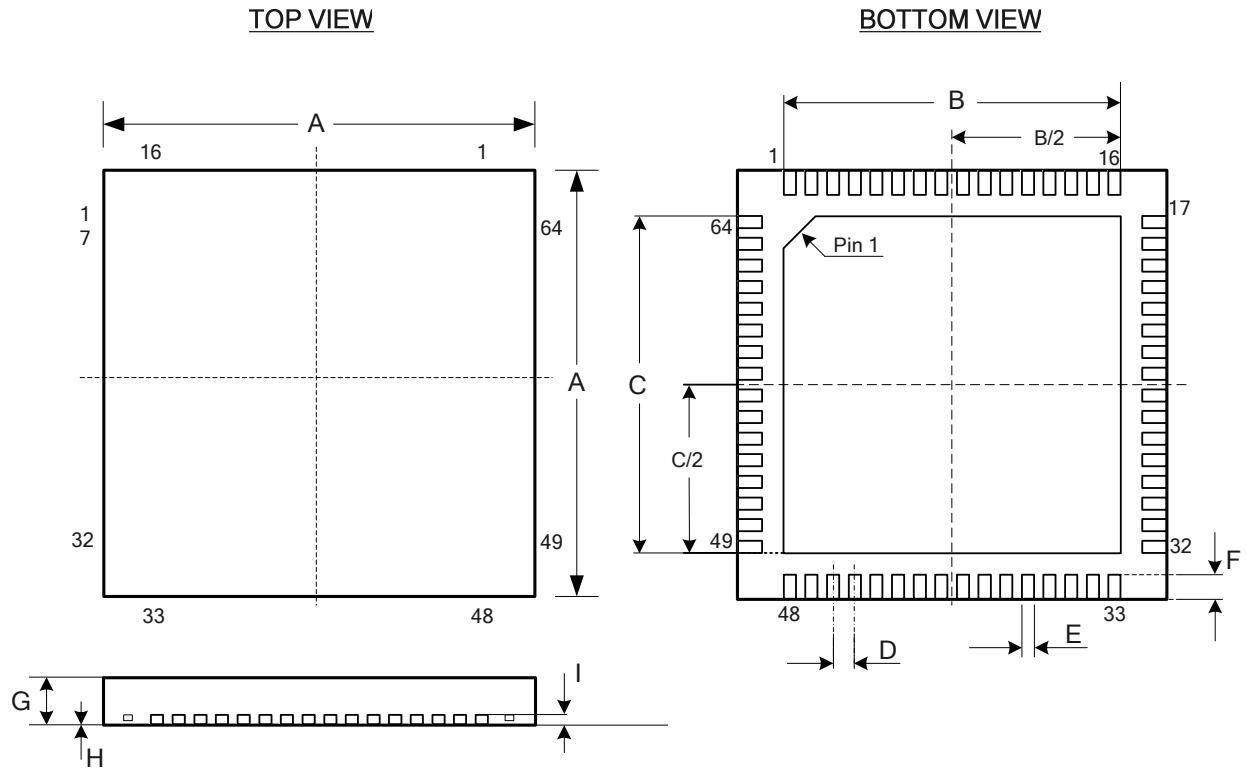
64 Pin QFN Package (8 x 8 x 0.8mm)
